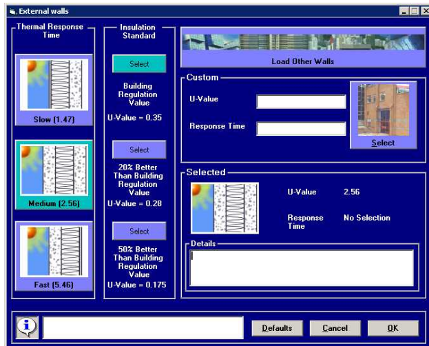
FIG. 6: External walls
